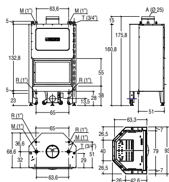
A Flue outlet; R System return; M System delivery; T System filling.
